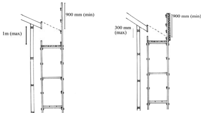
Figure 5a Fall arresting platform \leq 26^\circ
